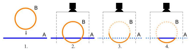
Figure 2: (1) A and B prior to collision. (2) Orthographic camera setup used to compute deformations on the GPU. (3) Back faces of B . (4) Front faces of A that penetrate B .
