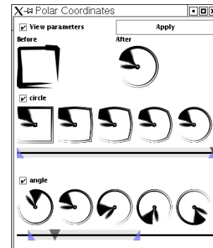
Figure 3. Side Views automatically generate previews of multiple, potential, future states, as in this example for a polar coordinates filter. For each parameter, an adjustable range of values is previewed via five images
